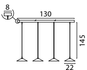
2151-15-15-130-4-22 Cacao Fixt. Cacao Sha- de, Black cable, 4x 12W 4x 1440Lm 2700-2200K, Triac-Dim.
