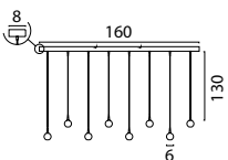
2411-37-37-160-8 Nickel Fixt. Nickel Shade, 8x 4,4W 8x 450Lm 3000- 2200K, Triac-Dim.
