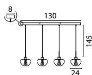
2971-05-05-130-4-24 Black Fixt. Black Cover, PVC cable, 4x E27 max 18W Bulb excl.
