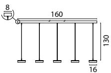
2041-05-81-02-160-5 Black Fixt. Black Cover, PVC cable, 5x 8W 5x 960Lm 2700-2200K, Triac-Dim.
