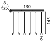
2411-05-05-130-6 Black Fixt. Black Shade, 6x 4,4W 6x 450Lm 3000- 2200K, Triac-Dim.
