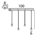
2411-05-02-100-4 Black Fixt. Gold Shade, 4x 4,4W 4x 450Lm 3000- 2200K, Triac-Dim.
