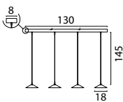
2151-37-37-130-4-18 Nickel Fixt. Nickel Shade, Transparent cable, 4x 8W 4x 960Lm 2700-2200K, Triac-Dim.
