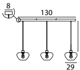
2971-05-05-130-3-29 Black Fixt. Black Cover, PVC cable, 3x E27 max 18W Bulb excl.
