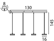
2041-37-37-02-130-4 Nickel Fixt. Nickel Cover, PVC cable, 4x 8W 4x 960Lm 2700-2200K, Triac-Dim.
