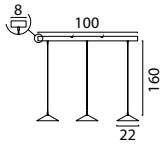
2151-1013-1013100322 White Fixt. White Shade, Transparent cable, 3x 12W 3x 1440Lm 2700- 2200K, Triac-Dim.
